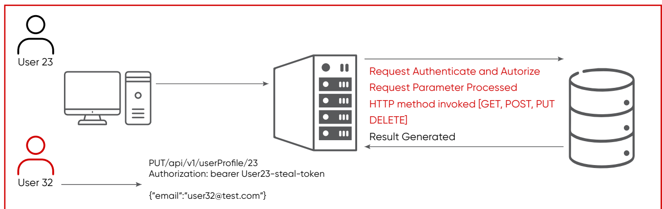
Fig.4: Broken User Authentication: Account takeover process, User32 can steal User23's token and update his mail in a password reset scenario.
