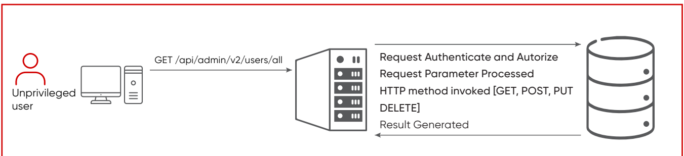
Fig 7: User32, an unprivileged user, can access admin functions.
