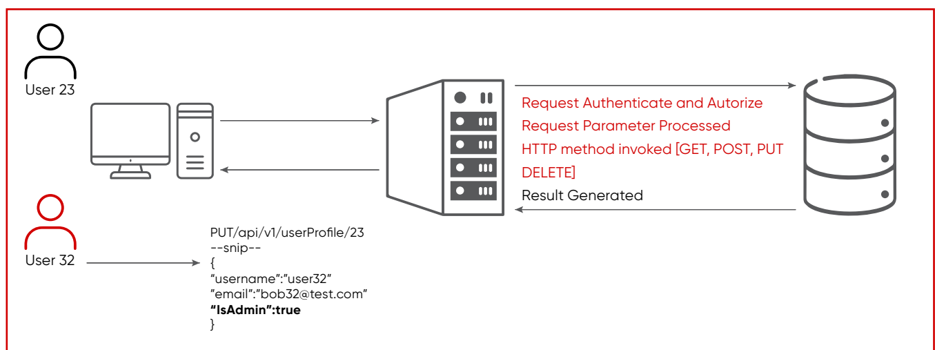
Fig 5: Unauthorized user32 can make himself admin.
