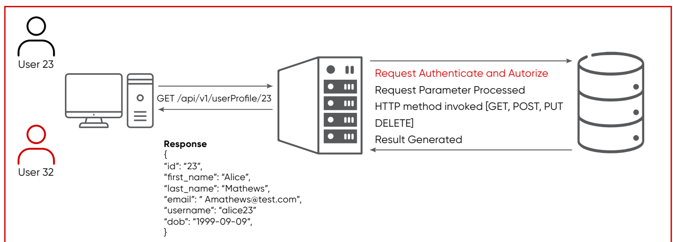
Fig.3: Broken Object Level Authorization: User32 can access User23's user profile
